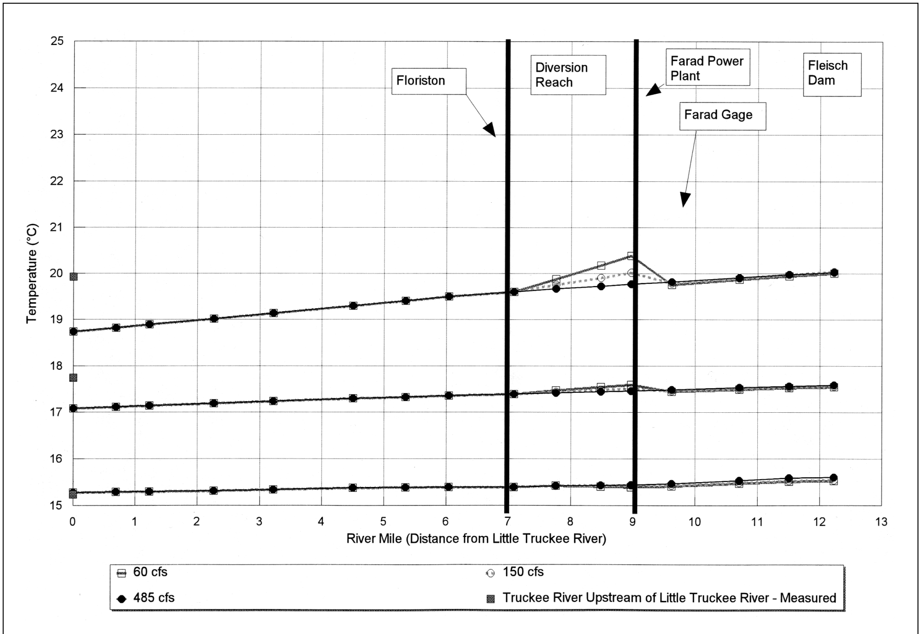
Figure 4-1 Simulated Average Daily Minimum, Mean, and Maximum Temperatures in the Truckee River for July and August; Flows Reduced from 485 cfs to 60, 150, and 485 cfs in the Floriston Diversion Reach
