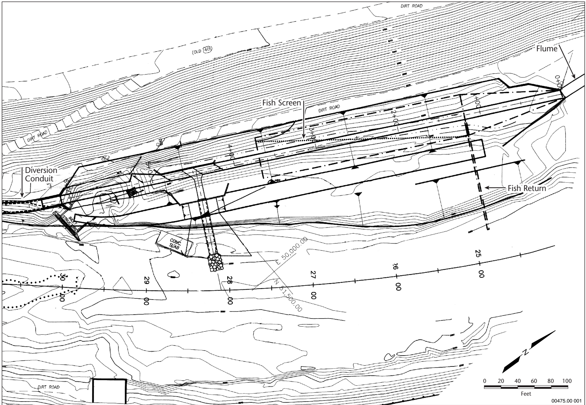
Figure 2-6 Fish Screen and Return
