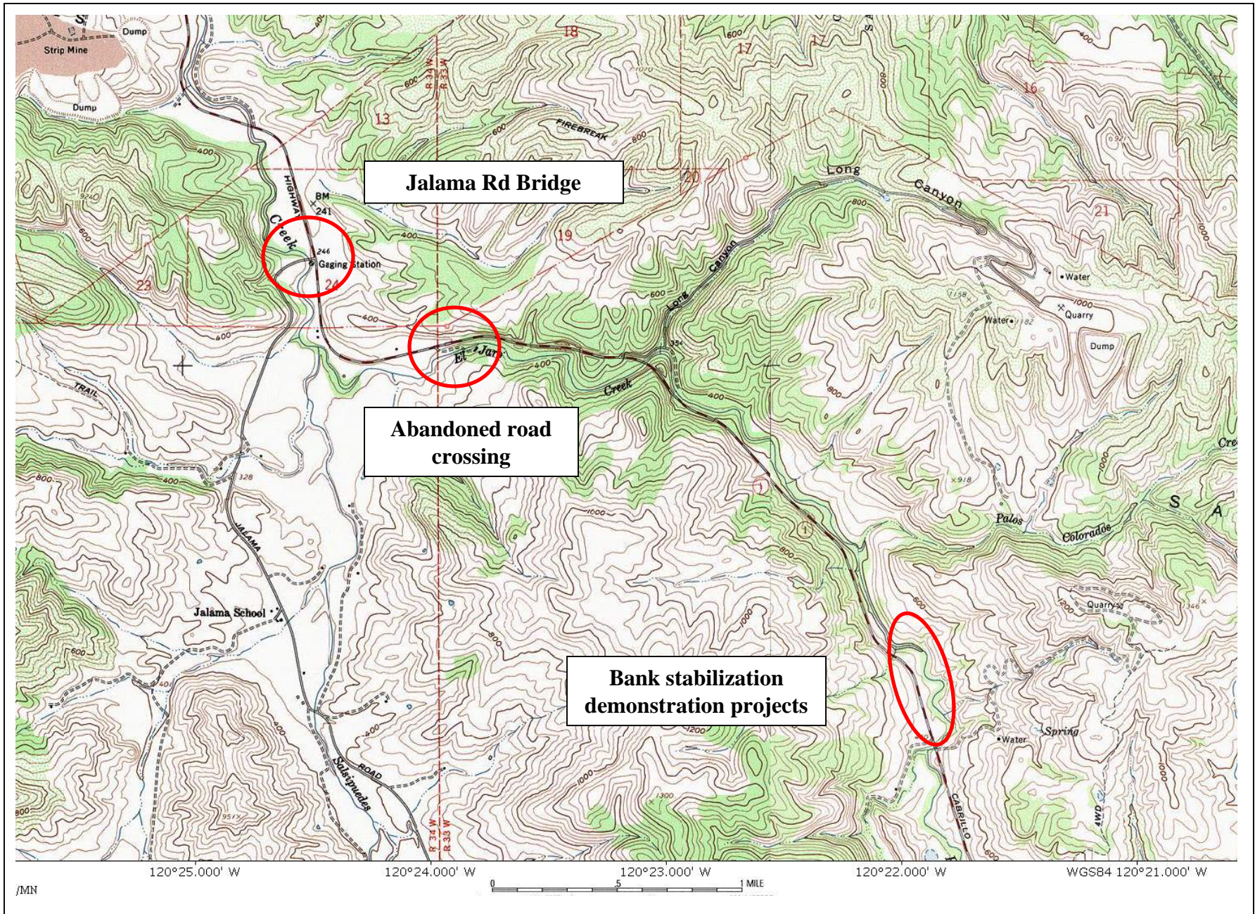
Figure 2-7. Locations of Jalama Road Bridge and EL Jaro Creek Projects
