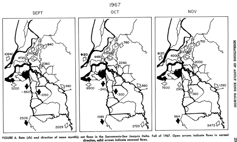
FIGURE 6. Rate (cfs) and direction of mean monthly net flows in the Sacramento-San Joaquin Delta. Fall of 1967. Open arrows indicate flows in normal direction, solid arrows indicate reversed flows.
