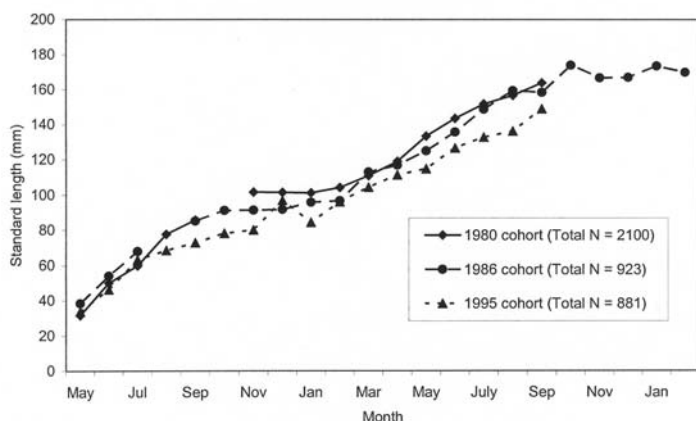
Growth of three splittail cohorts in Suisun Marsh
