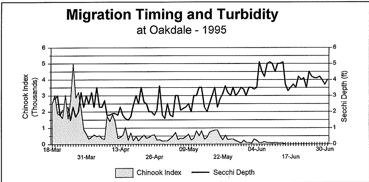
Figure 7. Comparison of the daily abundance index for chinook outmigrants to the river turbidity at Oakdale, 1995.
