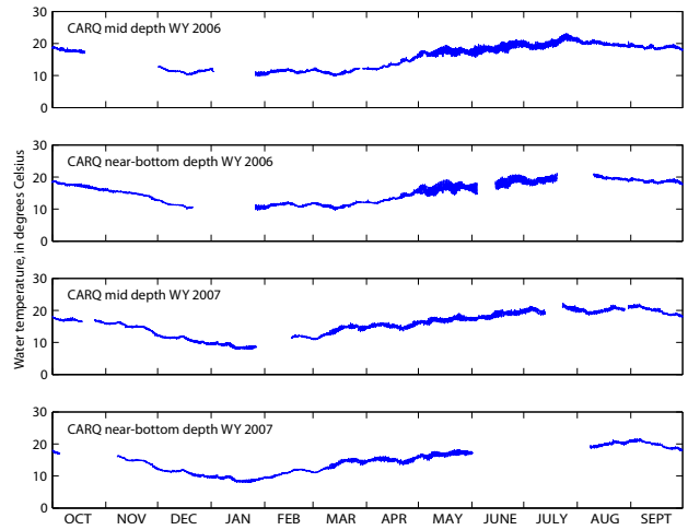
Figure 9 Measurements of water temperature at Carquinez Bridge (CARQ), San Pablo Bay, water years 2006, 2007
