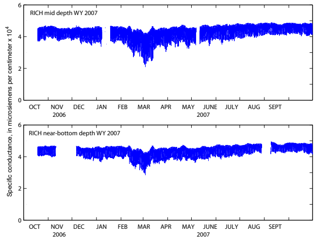
Figure 5 Measurements of specific conductance at Richmond/San Rafael Bridge (RICH), Central San Francisco Bay, water year 2007. For reference, seawater has a specific conductance of about 53,000 microsiemens per centimeter ( 5.3 \times 10^4 )
