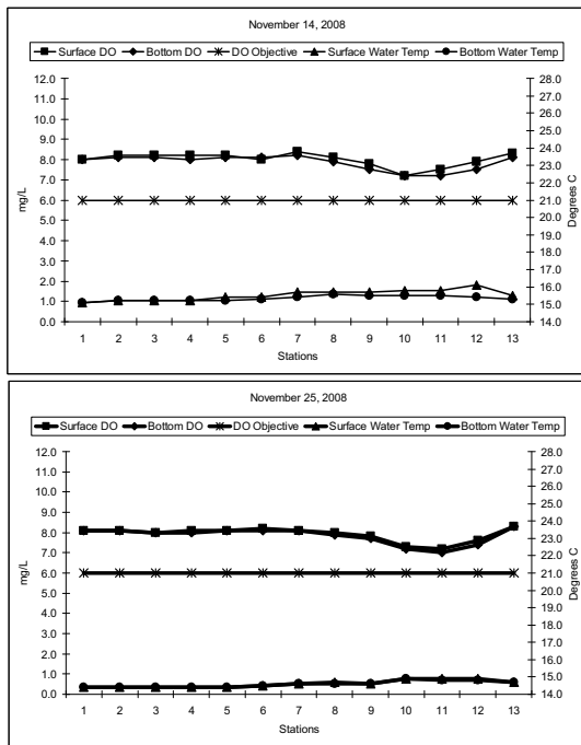
Figure 8 DO and water temperature during two monitoring cruises in November 2008
