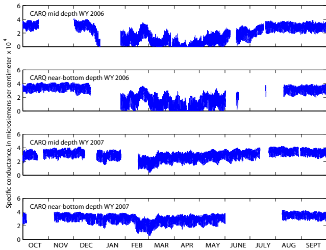
Figure 3 Measurements of specific conductance at Carquinez Bridge (CARQ), San Pablo Bay, water years 2006, 2007. For reference, seawater has a specific conductance of about 53,000 microsiemens per centimeter ( 5.3 \times 10^4 )
