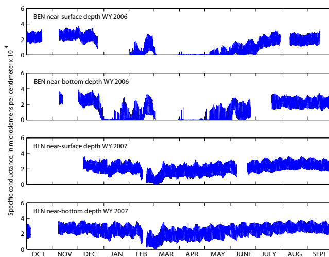
Figure 2 Measurements of specific conductance at Benicia Bridge (BEN), Suisun Bay, water years 2006, 2007. For reference, seawater has a specific conductance of about 53,000 microsiemens per centimeter ( 5.3 \times 10^4 ).
