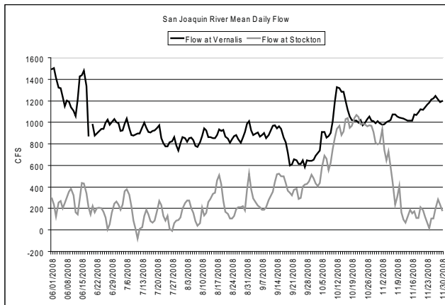
Figure 2 San Joaquin River mean daily flow
