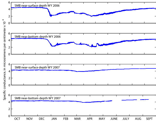
Figure 7 Measurements of specific conductance at San Mateo Bridge (SMB), South San Francisco Bay, water years 2006, 2007. For reference, seawater has a specific conductance of about 53,000 microsiemens per centimeter ( 5.3 \times 10^4 )
