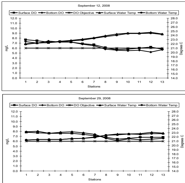
Figure 6 DO and water temperature during two monitoring cruises in September 2008
