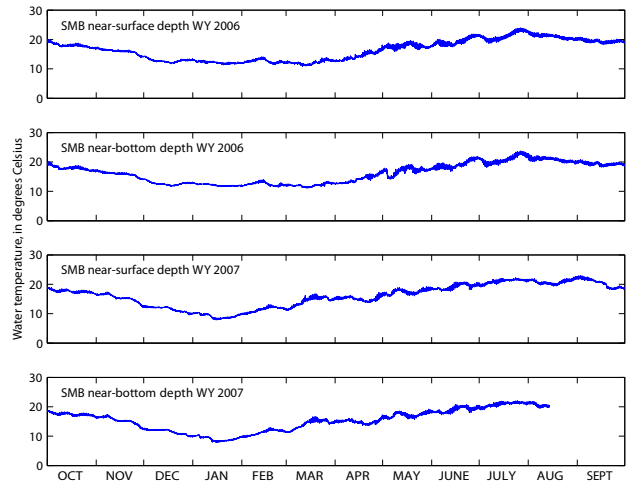
Figure 13 Measurements of water temperature at San Mateo Bridge (SMB), South San Francisco Bay, water years 2006, 2007
