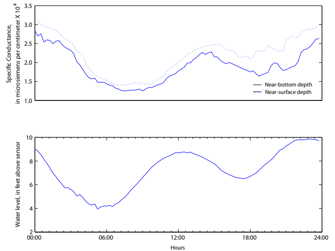
Figure 14 Near-surface and near-bottom measurements of specific conductance and water levels at Benicia Bridge, Suisun Bay, August 6, 2006. For reference, seawater has a specific conductance of about 53,000 microsiemens per centimeter ( 5.3 \times 10^4 )
