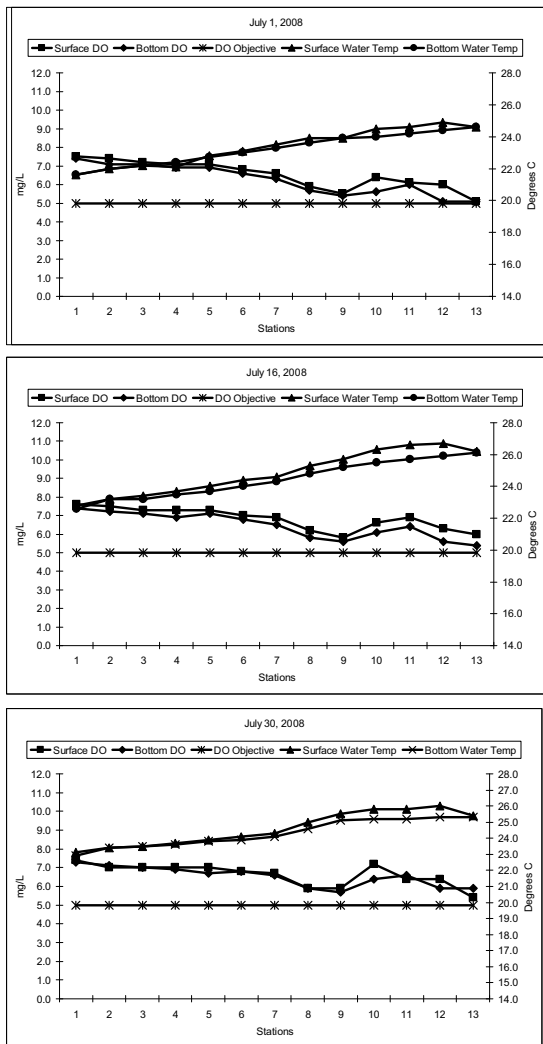
Figure 4 DO and water temperature during three monitoring cruises in July 2008
