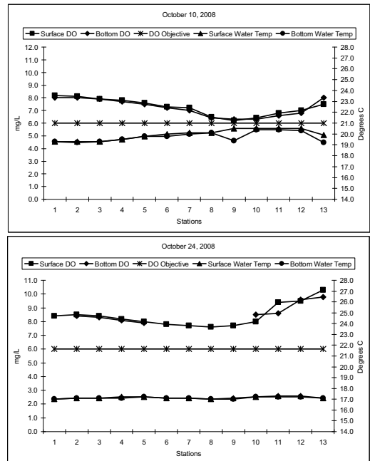
Figure 7 DO and water temperature during two monitoring cruises in October 2008
