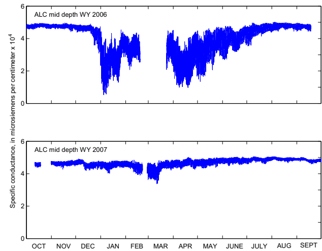
Figure 6 Measurements of specific conductance at Alcatraz Island (ALC), Central San Francisco Bay, water years 2006, 2007. For reference, seawater has a specific conductance of about 53,000 microsiemens per centimeter ( 5.3 \times 10^4 )
