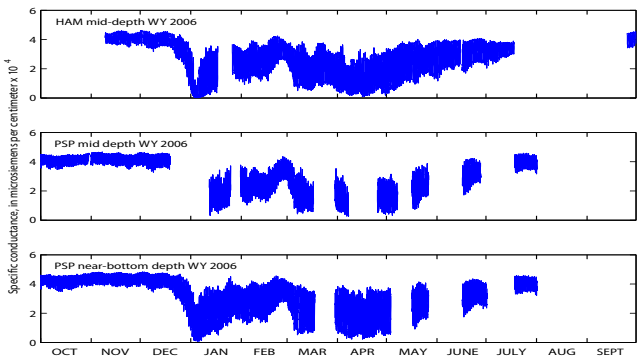
Figure 4 Measurements of specific conductance at Hamilton Disposal Site (HAM), and, Point San Pablo (PSP), San Pablo Bay and Central San Francisco Bay, respectively, water year 2006. For reference, seawater has a specific conductance of about 53,000 microsiemens per centimeter ( 5.3 \times 10^4 )
