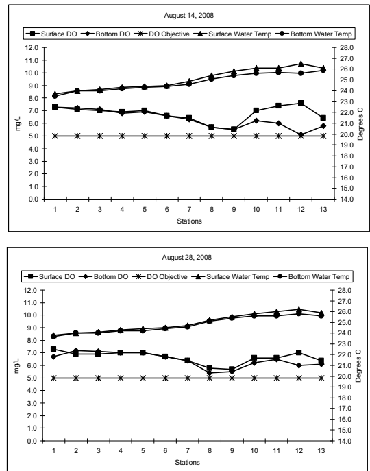
Figure 5 DO and water temperature during two monitoring cruises in August 2008
