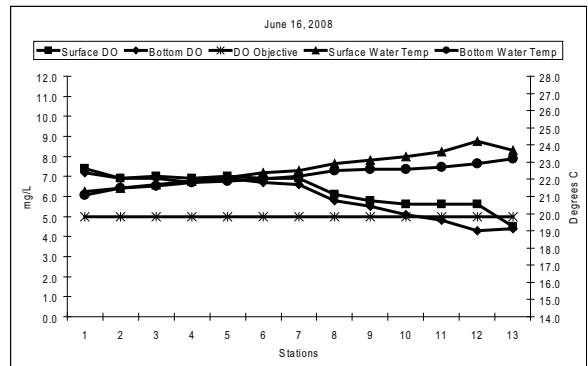
Figure 3 DO and water temperature during one monitoring cruise in June 2008
