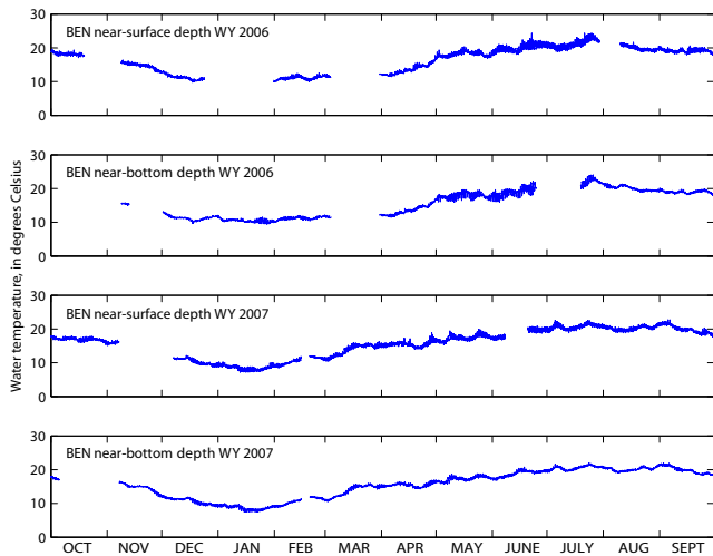
Figure 8 Measurements of water temperature at Benicia Bridge (BEN), Suisun Bay, water years 2006, 2007
