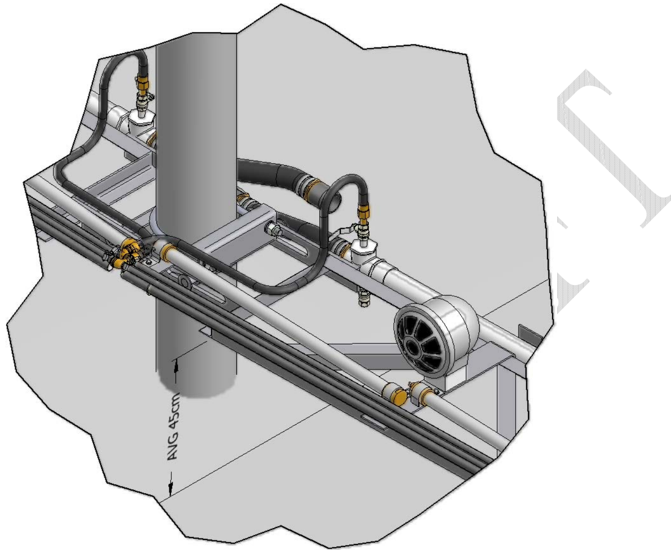
Figure 3. In this detailed drawing of the truss-style frame, with the BAFF components visible, the distance from the frame to the substrate is indicated as 45 cm. This was the space maintained between the BAFF components and the substrate along the entire 112 m of the BAFF.
