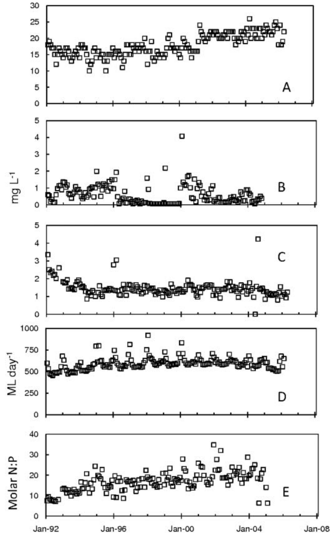
Figure 6 Nutrient concentrations ( \text{mg L}^{-1} ) of the wastewater effluent as a function of time for (A) \text{NH}_4^+ ; (B) \text{NO}_3^- + \text{NO}_2^- ; (C) \text{PO}_4^{3-} ; (D) the volumetric daily rate of effluent discharge ( \text{ML day}^{-1} ) from the wastewater facility; and (E) the molar ratio of dissolved inorganic nitrogen:phosphorus (DIN:DIP) for the major wastewater treatment facility in the upper Sacramento River. Although the plant came on line in 1982, the available data are only from 1992.
