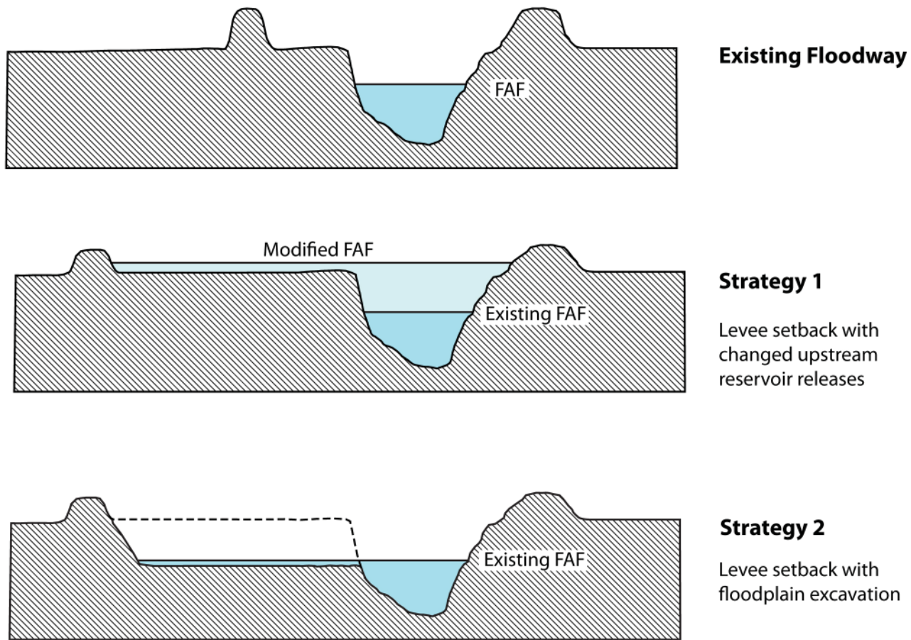
Figure 16 Two strategies for increasing "Activated Floodplain" area with levee setback
