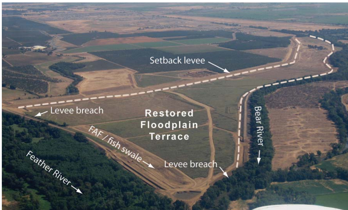
Figure 17 Bear River Levee Setback Project, design based on FAF approach
