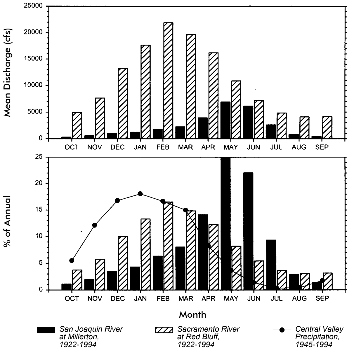
Figure II-C Average Monthly Unimpaired (Natural) Discharge from the Upland Sacramento and San Joaquin River Watersheds
