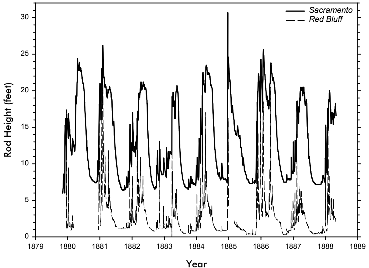
Figure II-J Modifying Effects of Flood Basin and Tributary Inflow on the Lowland Sacramento River Flow
