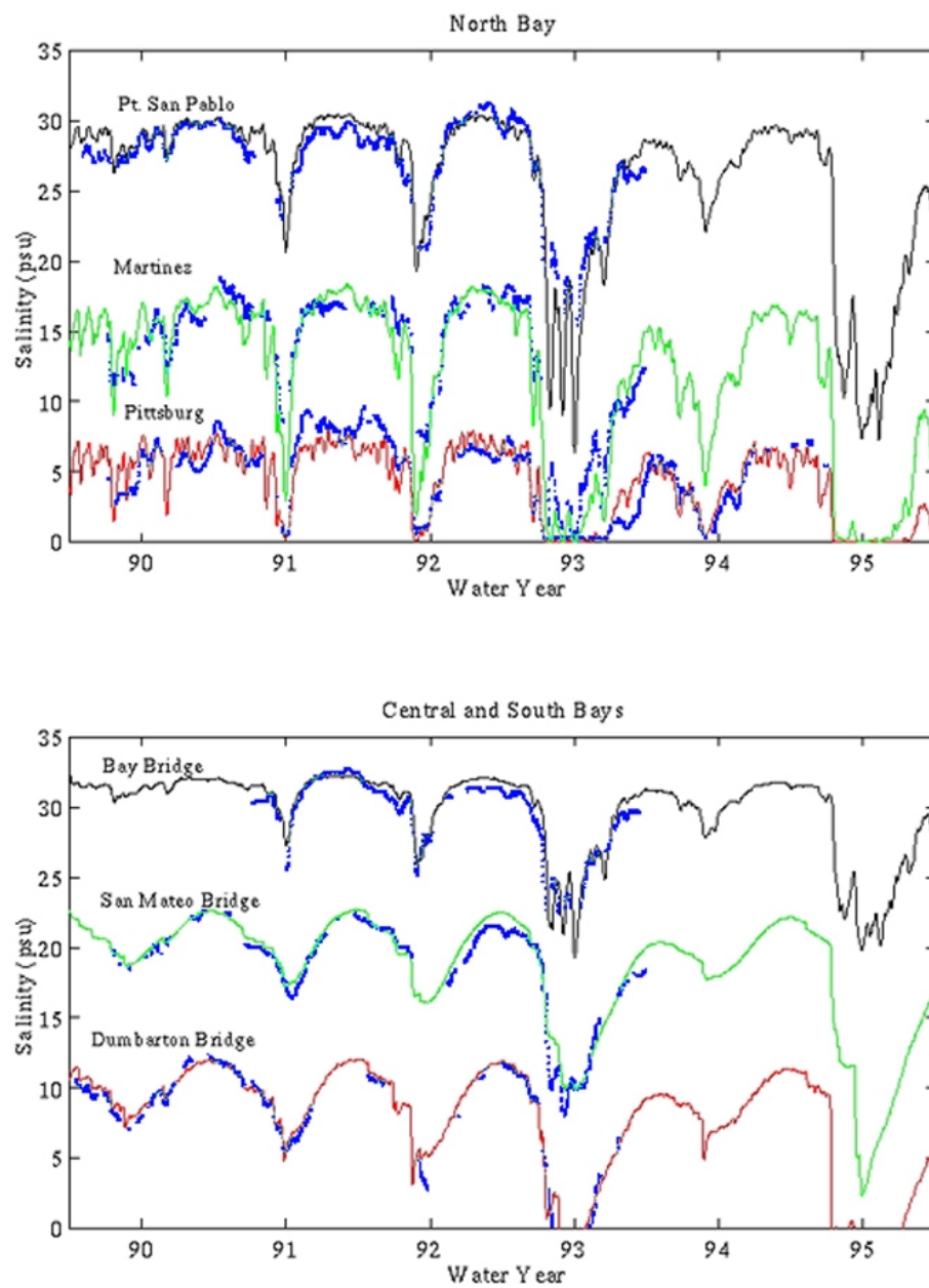
Figure 2.3 Simulated salinities (solid lines) and observations (blue dots) from several stations throughout the Bay. Observations at San Mateo and Dumbarton Bridges are offset by -10 psu and -15 psu , respectively.
