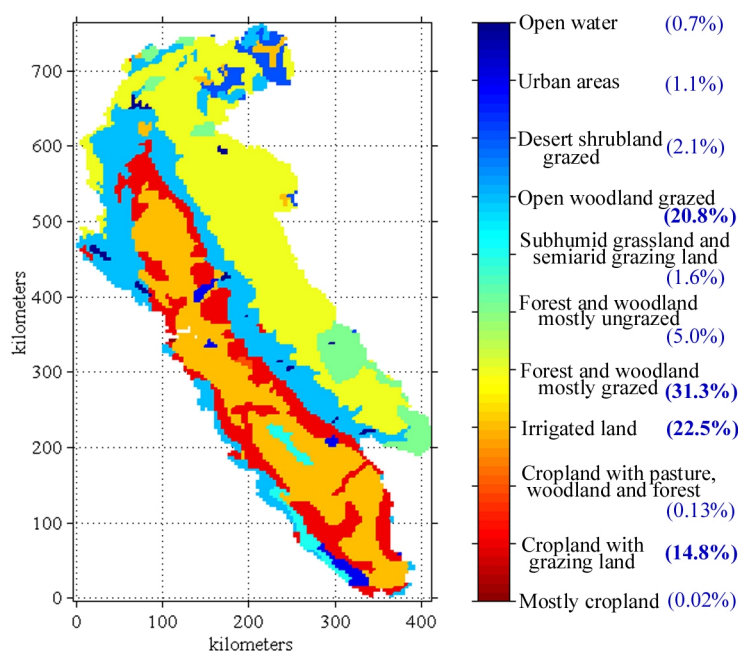
Figure 5.16 Land cover classifications of the watershed with percent area covered. The dominant categories are “cropland with grazing land”, “irrigated land”, “forest and woodland mostly grazed”, and “open woodland grazed”.
