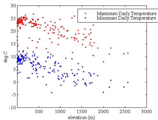
Figure 5.30 Mean maximum and minimum daily temperature versus sensor altitude.
