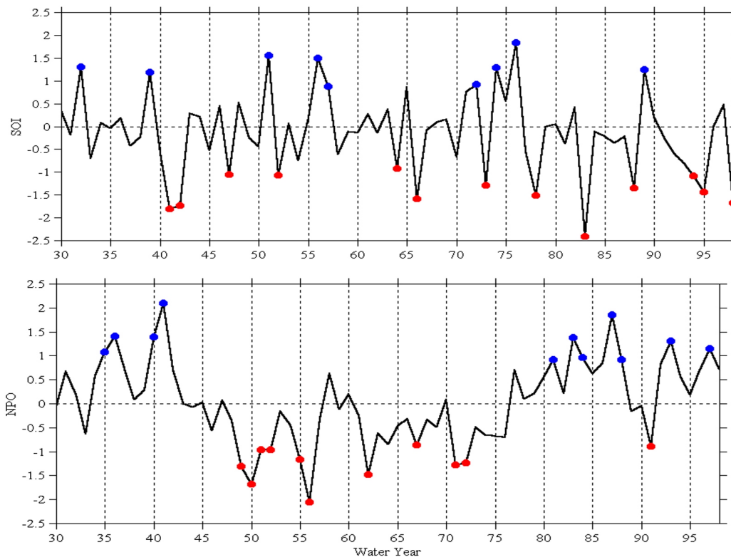
Figure 7.12 Annual values of SOI (top) and NPO (bottom) indices for WY 30-98. Values in excess of one standard deviation from the mean used for compositing are indicated.
