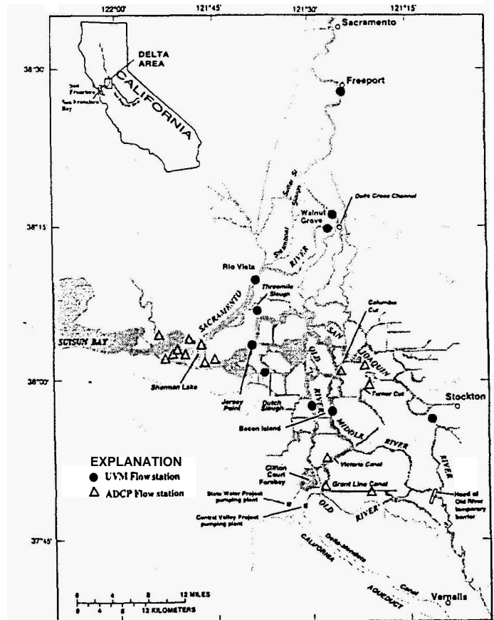
Figure 1 Map of the Delta showing the location of the current network of 10 UVM flow monitoring stations (solid circles). In situ acoustic Doppler current profilers (ADCP) have also been deployed for three month periods during the spring of 1996, 1997, and 1998 and the fall of 1998 (open triangles).
