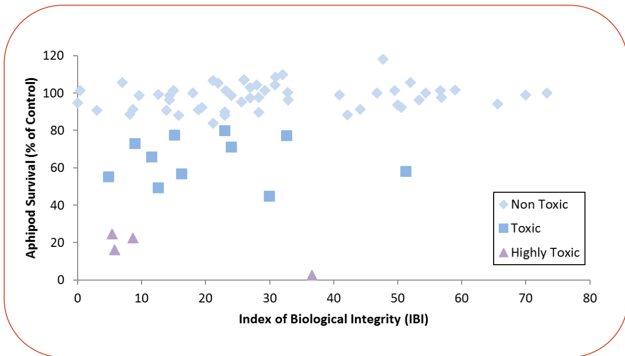
Figure 2. Relationship between amphipod survival in sediment toxicity tests and benthic macroinvertebrate Index of Biological Integrity scores. Amphipod survival is presented as a percentage of the respective control sample survival value.
