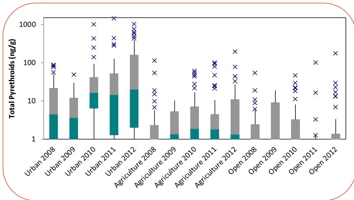
Figure 1. Total pyrethroid pesticide concentrations measured in sediments in relation to watershed land use in SPoT watersheds. Concentrations of pyrethroids increased between in all watersheds between 2008 and 2012, but most significantly in urban watersheds.
