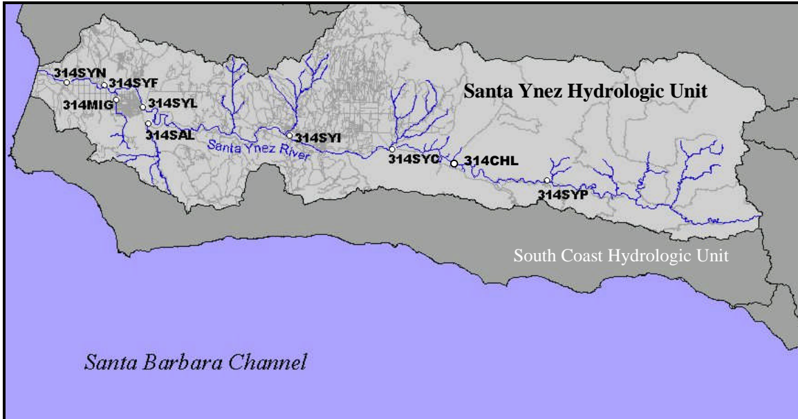
Figure 5.1a. CCAMP monitoring sites in the Santa Ynez Hydrologic Unit.
