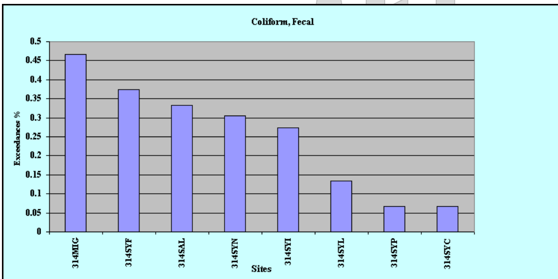
Figure 5.1.1a. Percent exceedance of the Basin Plan objective (400 MPN/100 ml) for fecal coliform at sites in the Santa Ynez Hydrologic Unit.
