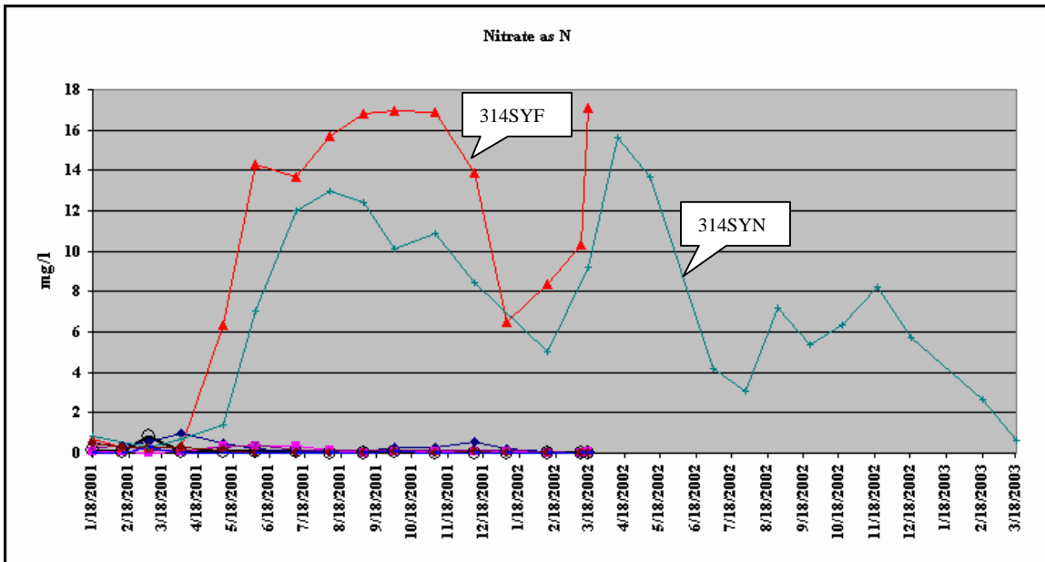
Figure 5.1.2a. Time series of nitrate levels at all sites in the Santa Ynez Hydrologic Unit between January 2001 and March 2003.
