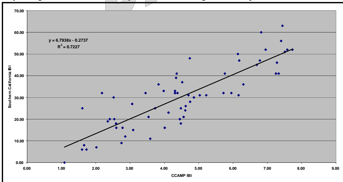
Figure B.1. Regression of Southern California Index of Biotic Integrity scores against Central Coast Ambient Monitoring Program Index of Biotic Integrity scores for the Central Coast Region.
