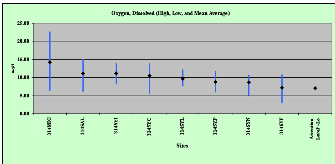
Figure 5.1.4a. Mean and range of dissolved oxygen levels (mg/L DO) at sites in the Santa Ynez River Hydrologic Unit between January 2001 and March 2002.
