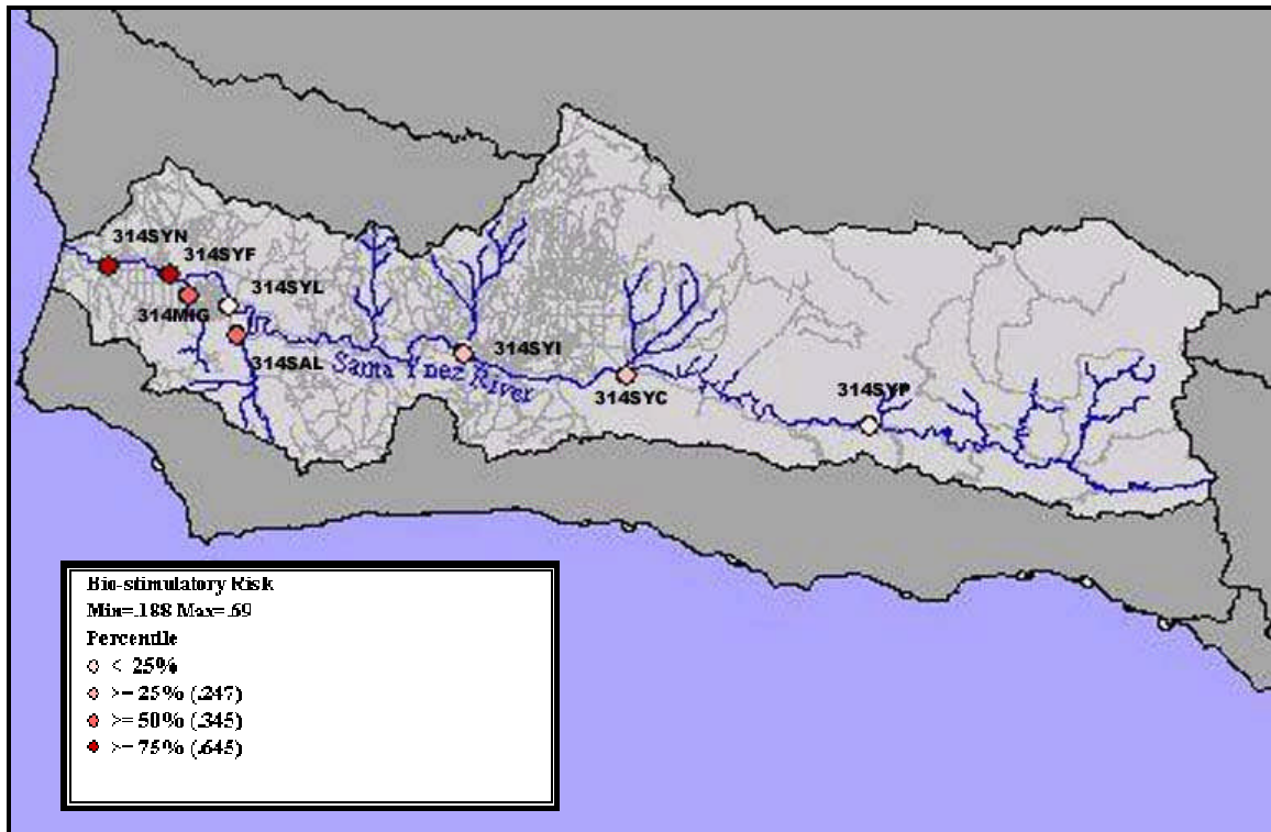
Figure 5.1.4b. Biostimulatory risk rankings at sites in the Santa Ynez Hydrologic Unit based on data collected between April 2001 and March 2002.
