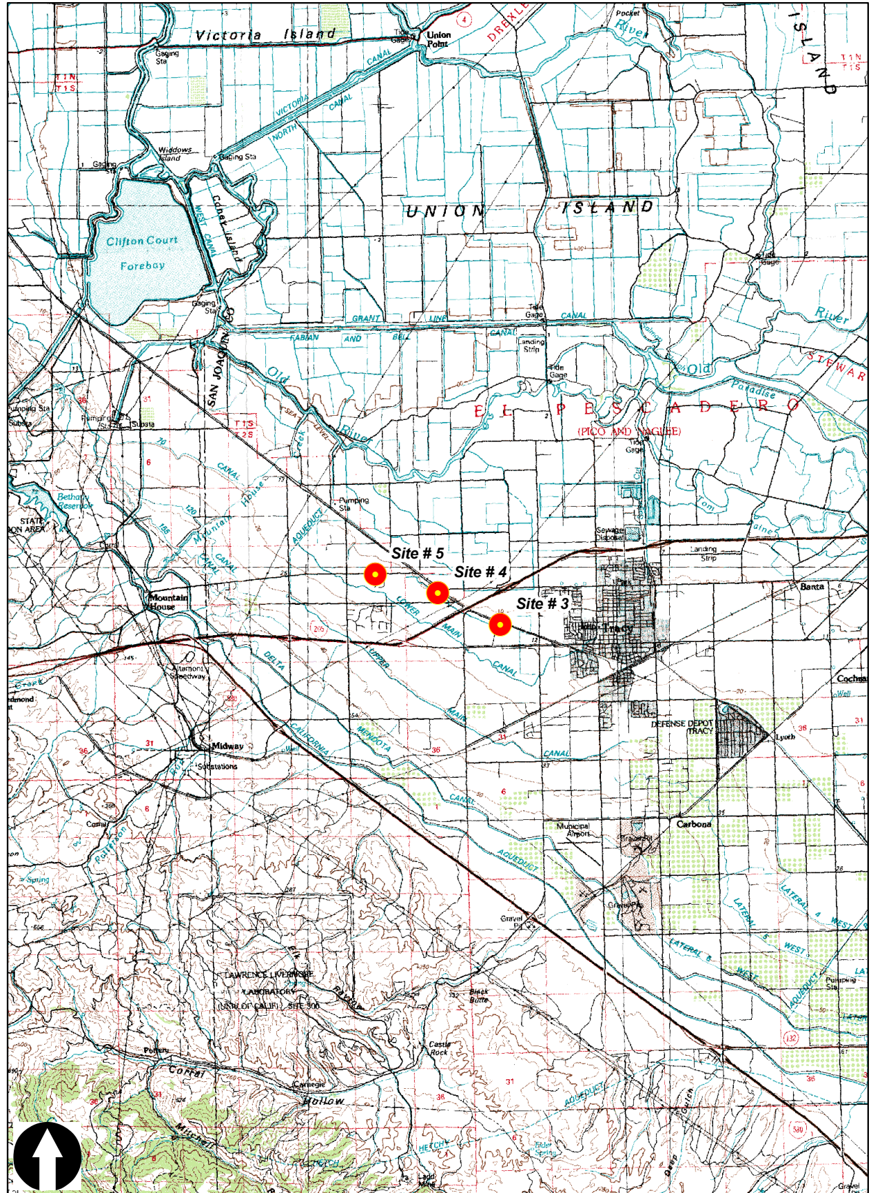
Figure 2 Sampling Sites for NPDES Annual Monitoring Report - Region 5 (South)
