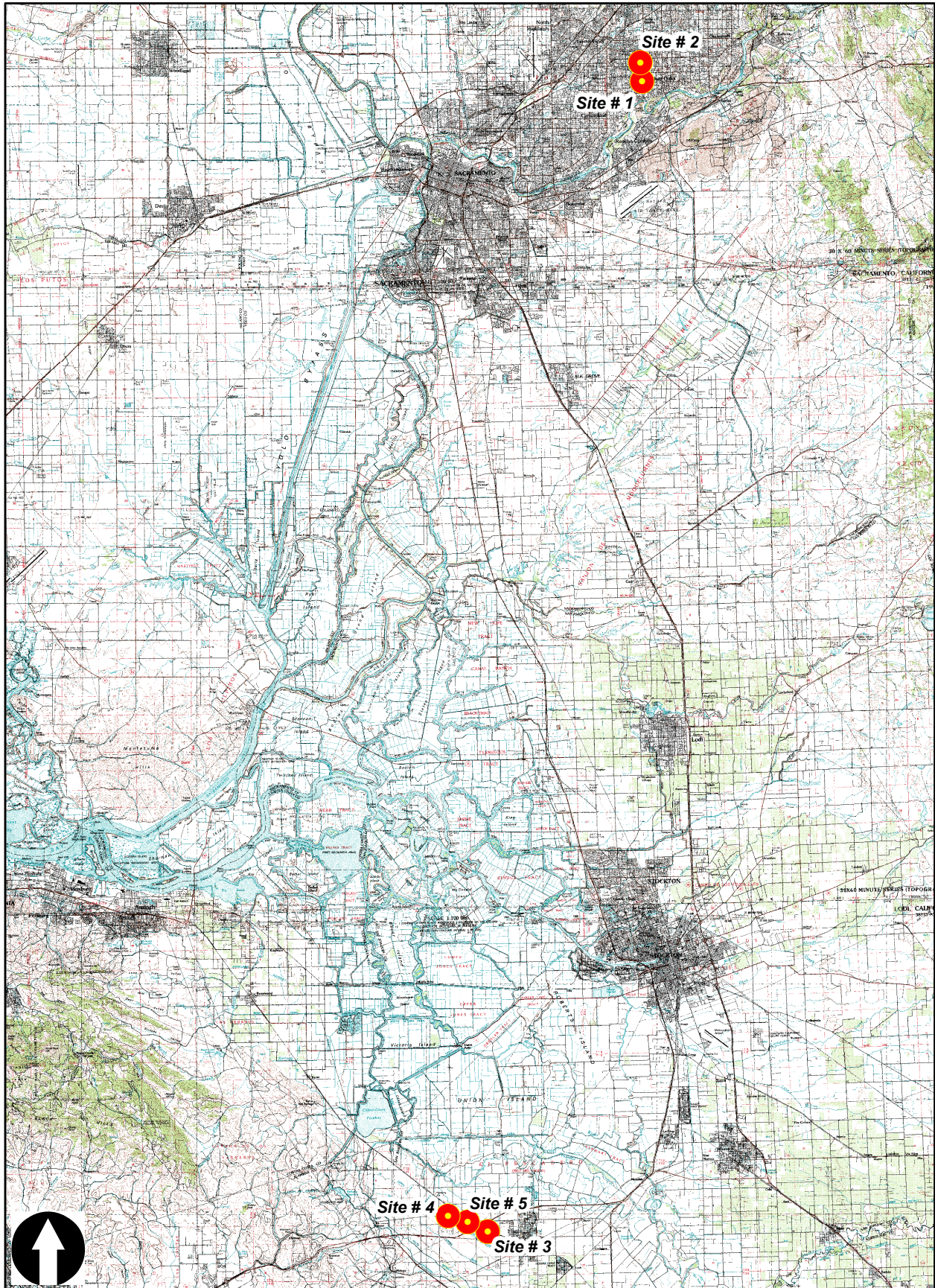
Figure 2. Sampling Sites for NPDES Annual Monitoring Report - Region 5
