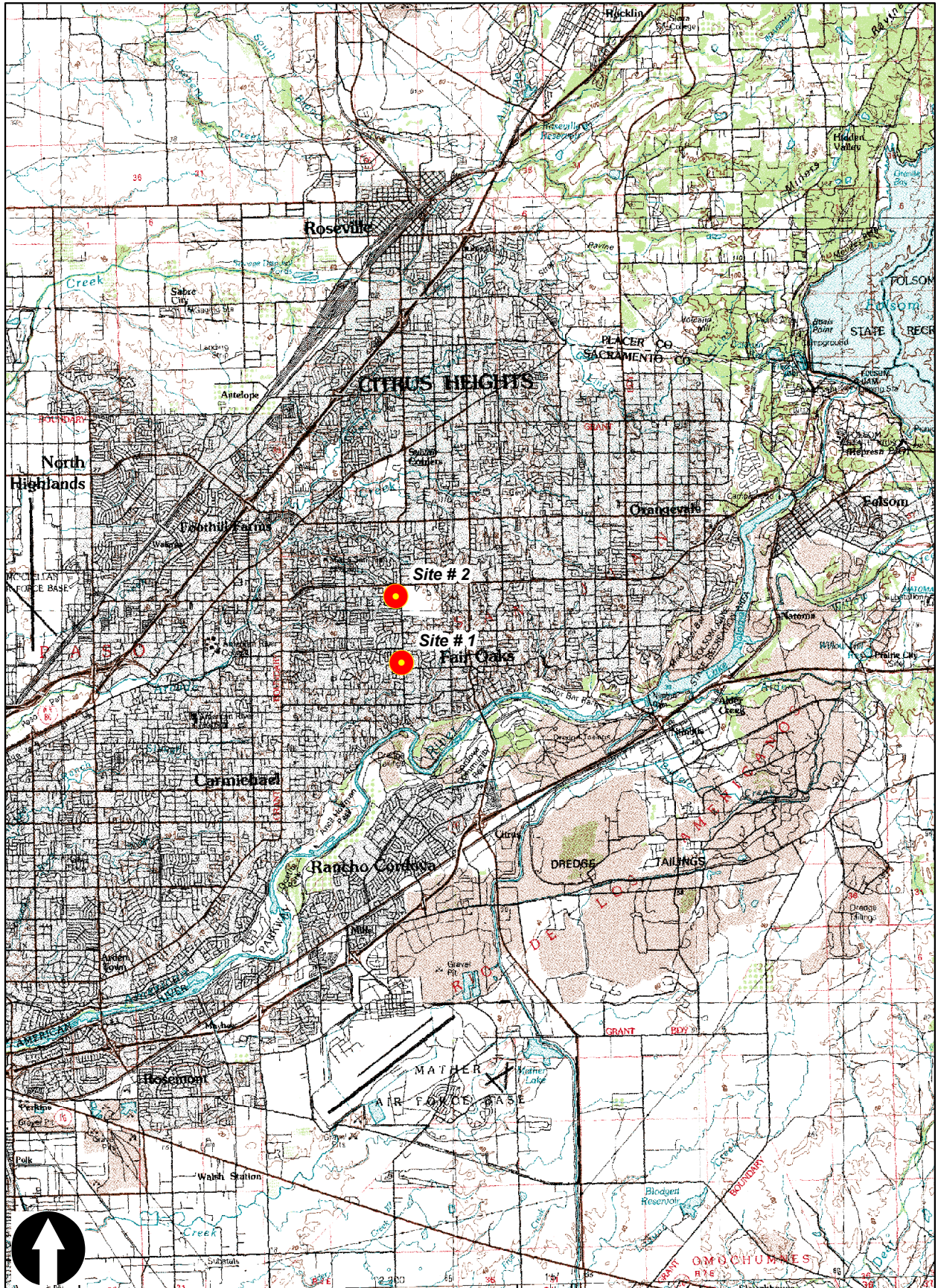
Figure 2 Sampling Sites for NPDES Annual Monitoring Report - Region 5 (North)
