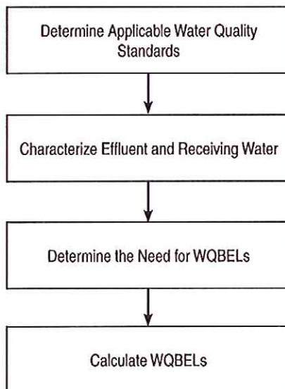
Exhibit 6-2 Standards-to-permits process
